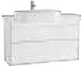
Washbasin unit, with drawers, 1TH, without overflow hole, 100cm Matt White & Natural Oak £2,466 – 62450 Flamed Grey & Natural Oak £2,466 – 62452 Sand & Taupe £2,466 – 62451 H: 550mm W: 1000mm P: 330mm (Ceramic vanity washbasin and waste cover included)
